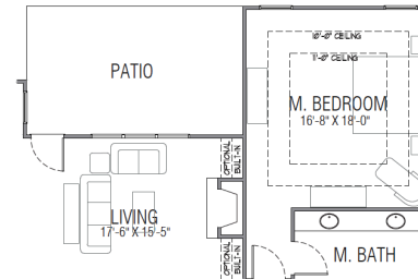
FIRST FLOOR PLAN @ OPT. EXT. MASTER LEXINGTON A
